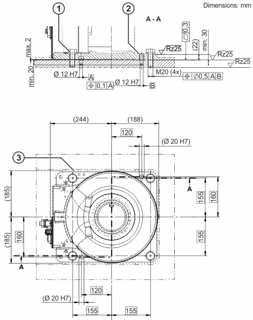
Fig. 5-5: Machine frame mounting, dimensioned drawing
